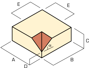
PL.35.24 Plinth internal return
